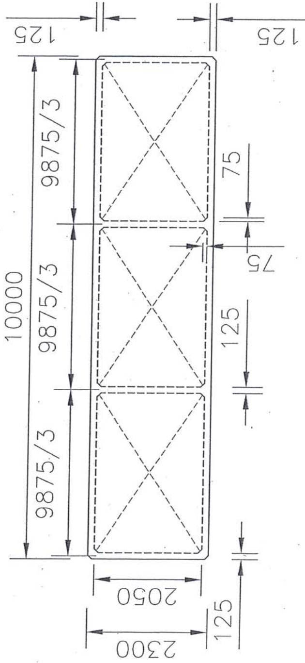
SECTION A-A: DIMENSION OF EACH SEGMENT (TYPICAL)
