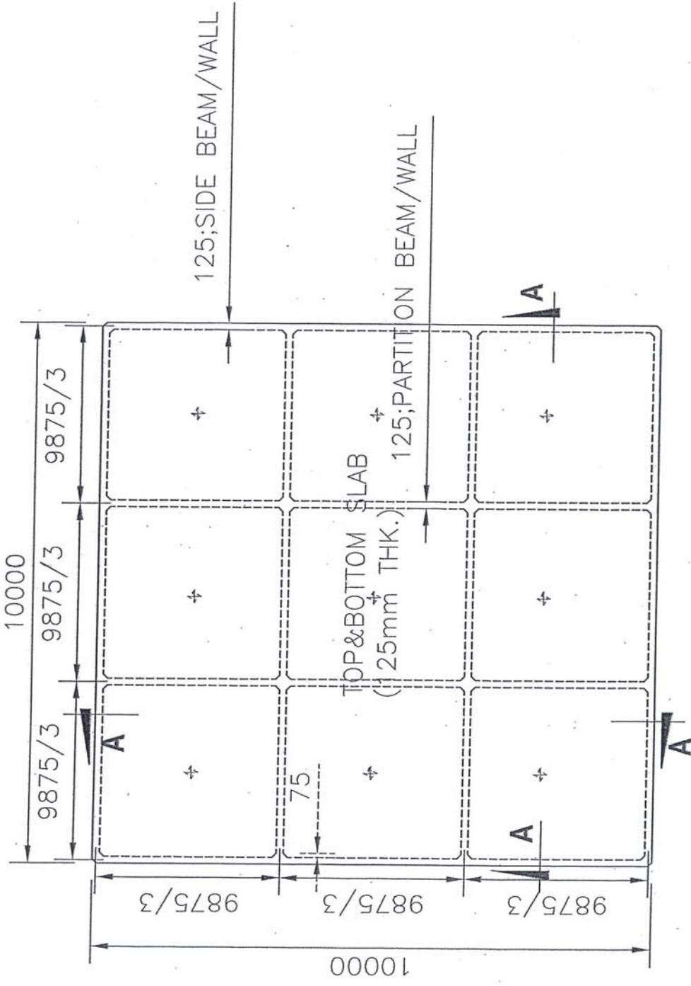
PLAN VIEW: DIMENSION OF EACH SEGMENT (TYPICAL)
